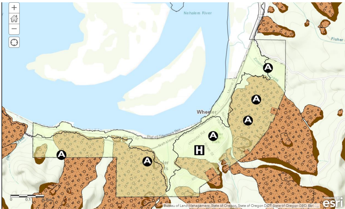
Figure 112. Landslide Deposits, Tsunami Evacuation Line, Assembly Areas, and a Critical Facility
