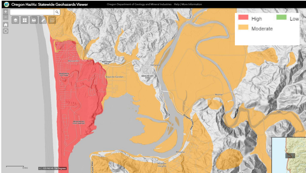
Figure 87. Liquefiable Soils in Bayside Gardens, Manzanita, Nehalem, and Wheeler
