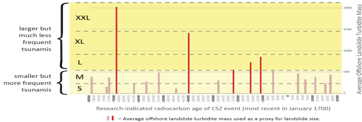
Figure 74. Occurrence and Relative Size of Cascadia Subduction Zone Megathrust Earthquakes
