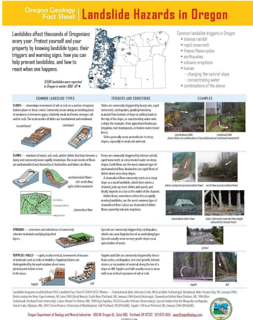
Figure 62. Common Types of Landslides in Oregon
