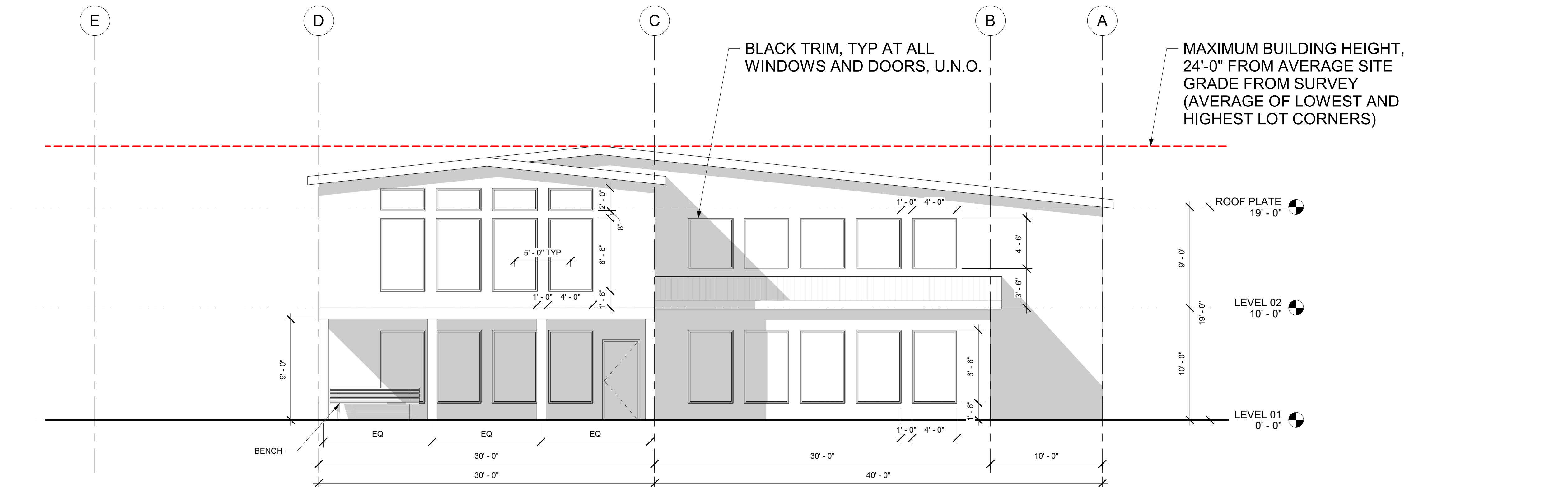
EXTERIOR - SOUTH ELEVATION 2 3/16" = 1'-0"
