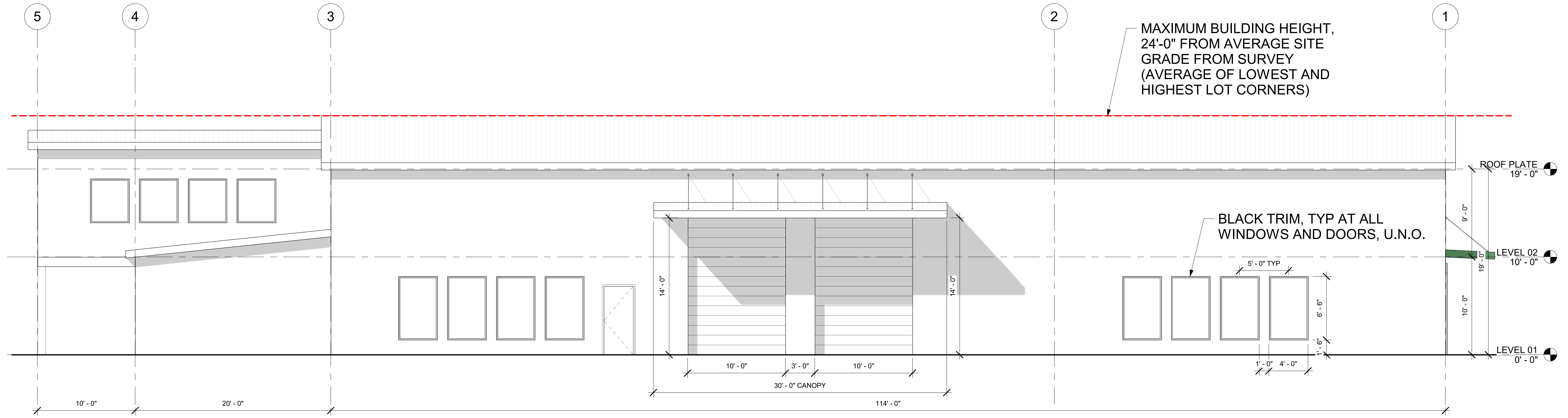
EXTERIOR - EAST ELEVATION 1 3/16" = 1'-0"
