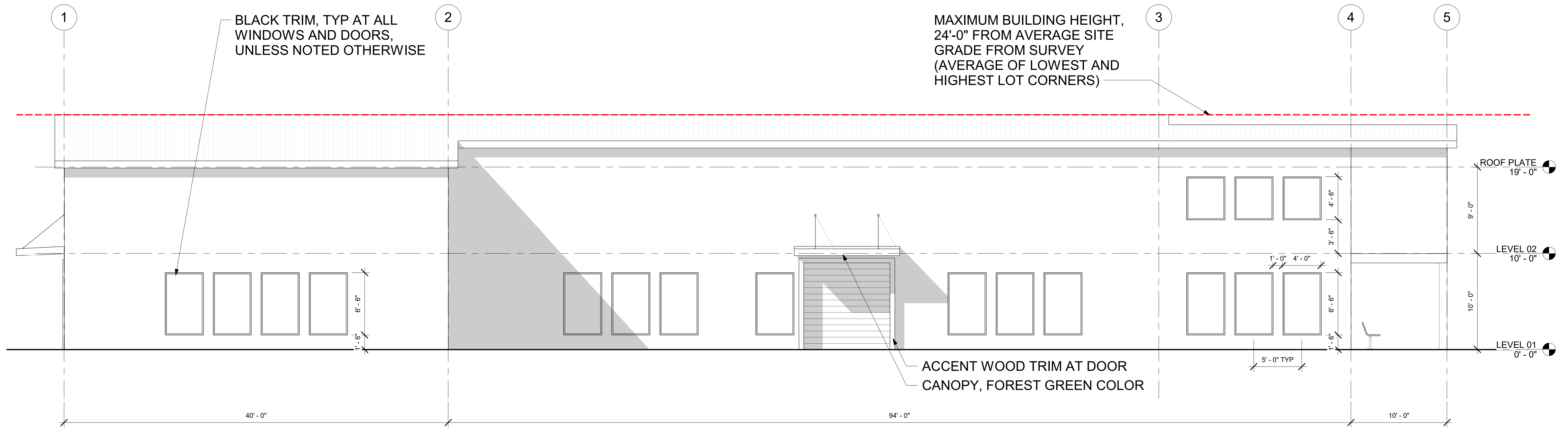
EXTERIOR - WEST ELEVATION ① 3/16" = 1'-0"
