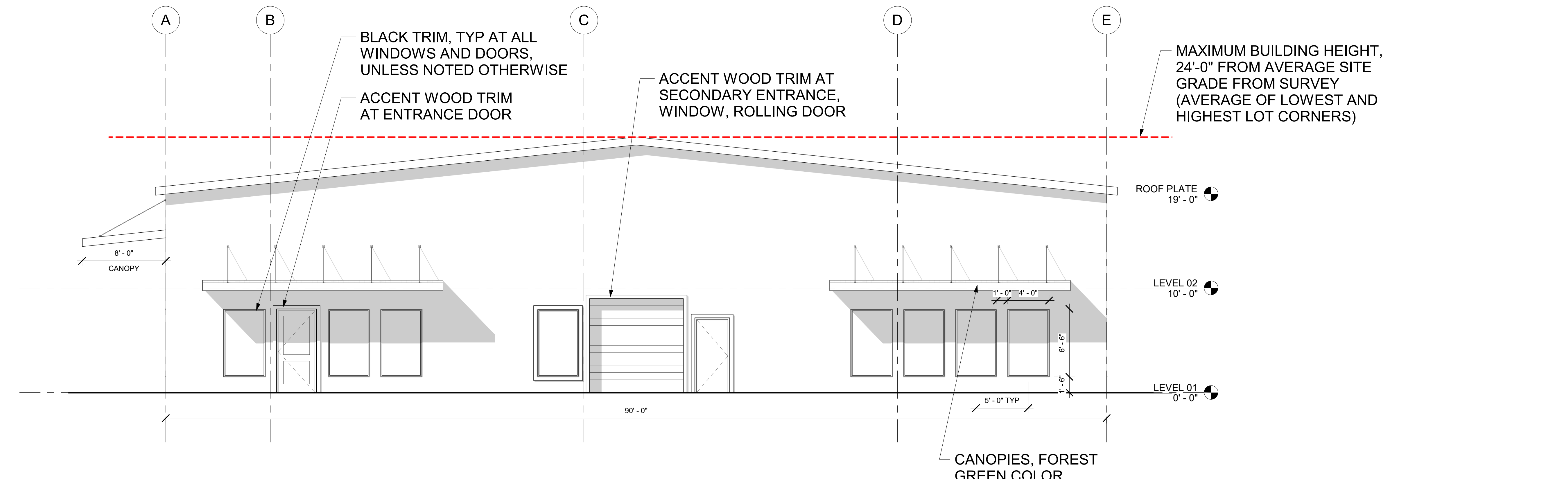
EXTERIOR - NORTH ELEVATION ② 3/16" = 1'-0"
