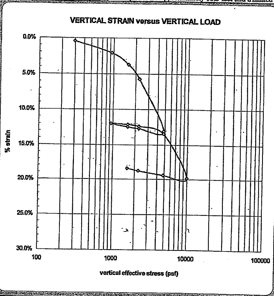
06176 S06-559 silt with sand - STRAIN PLOT, 9/15/2006
