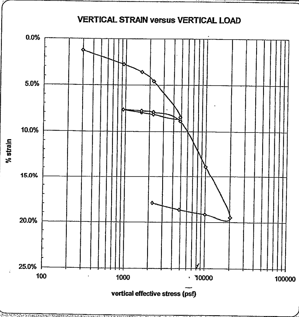
06176 S06-552 sandy silt - STRAIN plot, 8/25/2006
